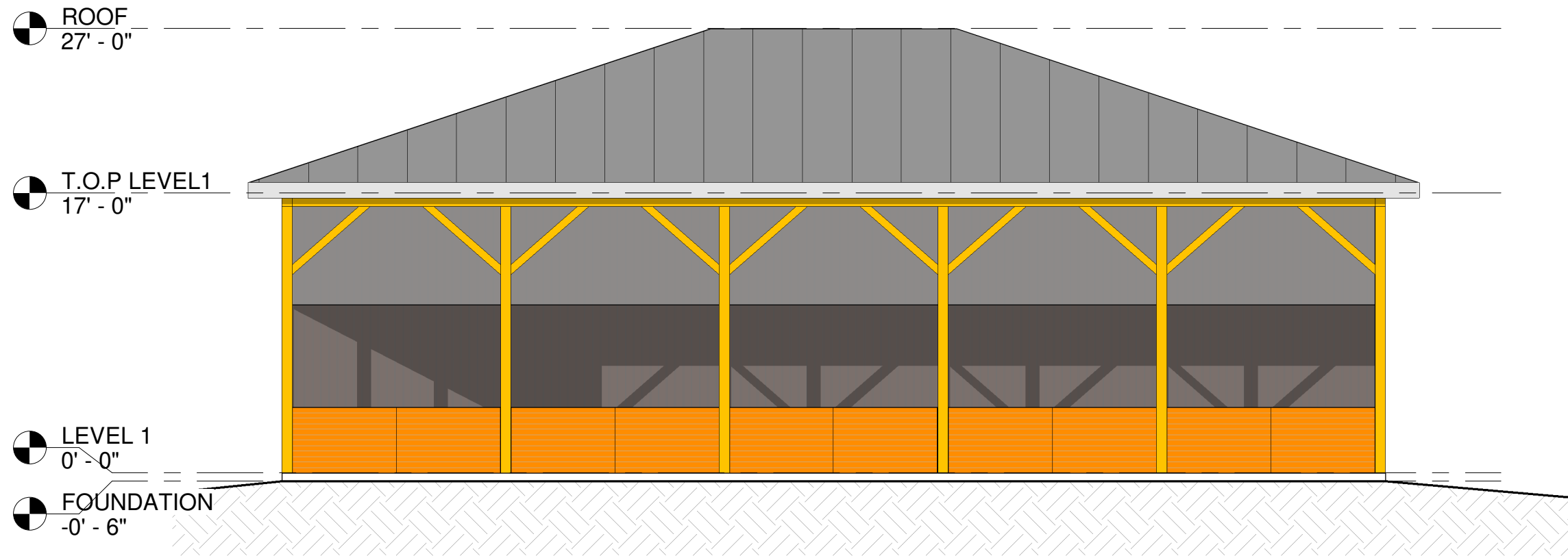
② WEST ELEVATION 1/8" = 1'-0"
