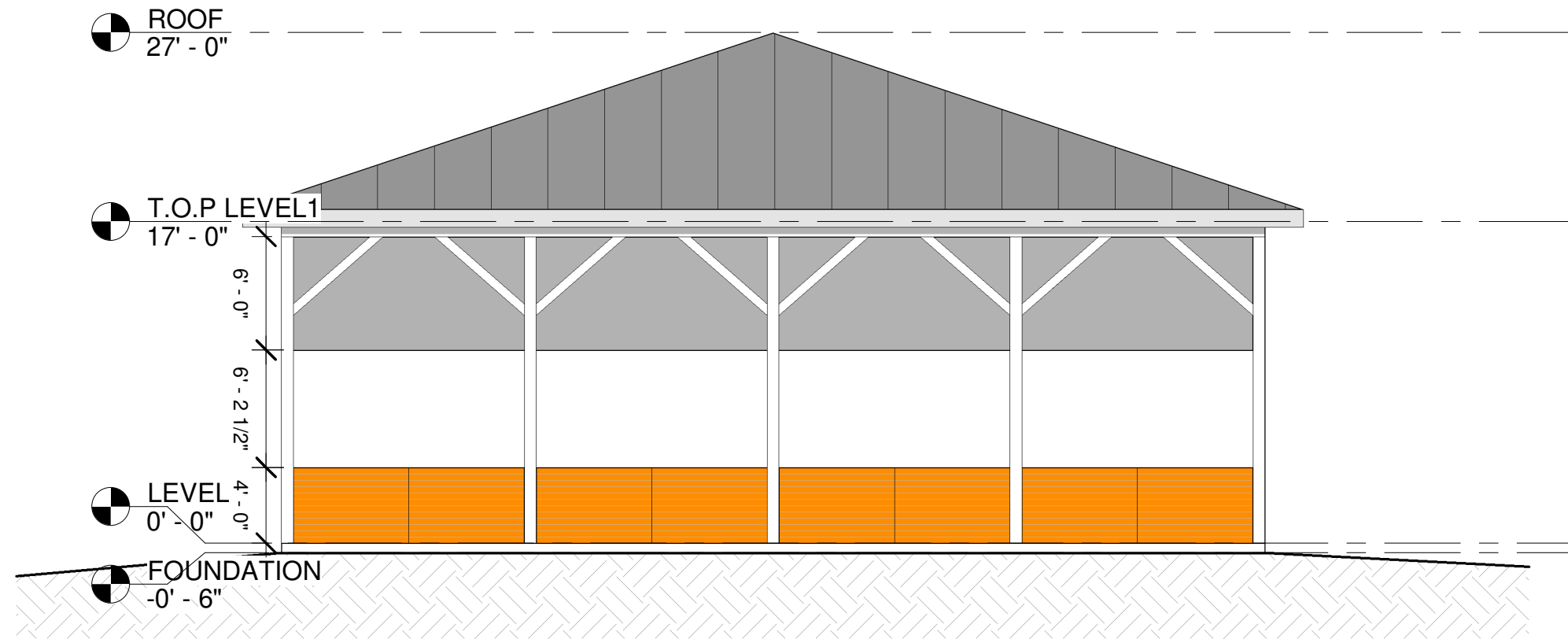
① SOUTH ELEVATION 1/8" = 1'-0"
